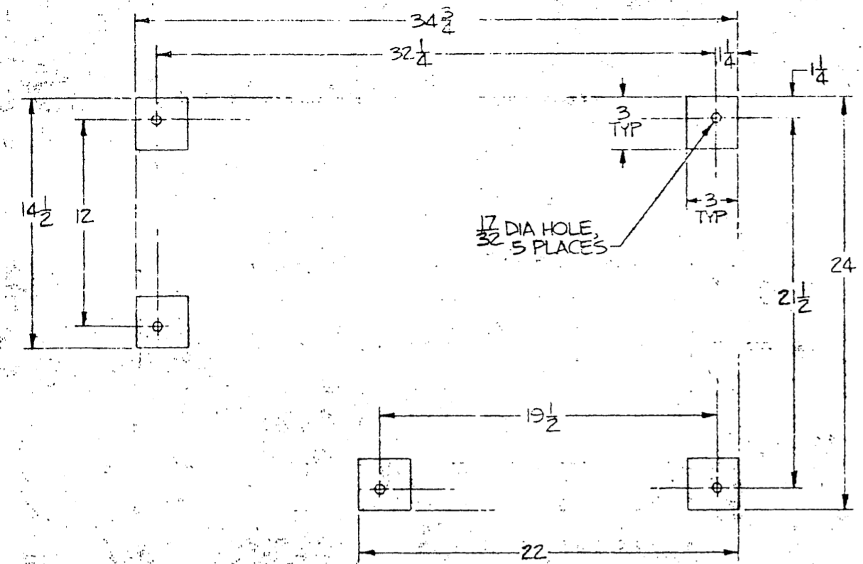
DECK BOLTING PLAN A-A
